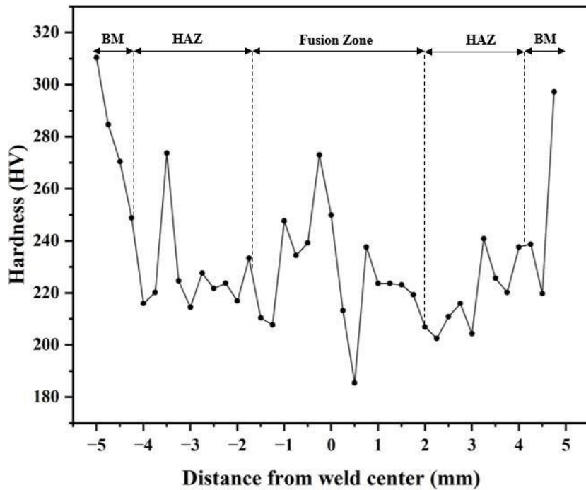
Figure 8: Microhardness profile along the transverse direction of TIG welded sample
