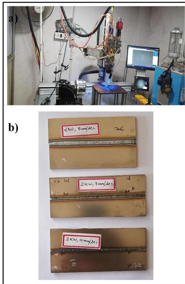
Figure 2: (a) Laser welding set-up (b) Laser Welded plates
