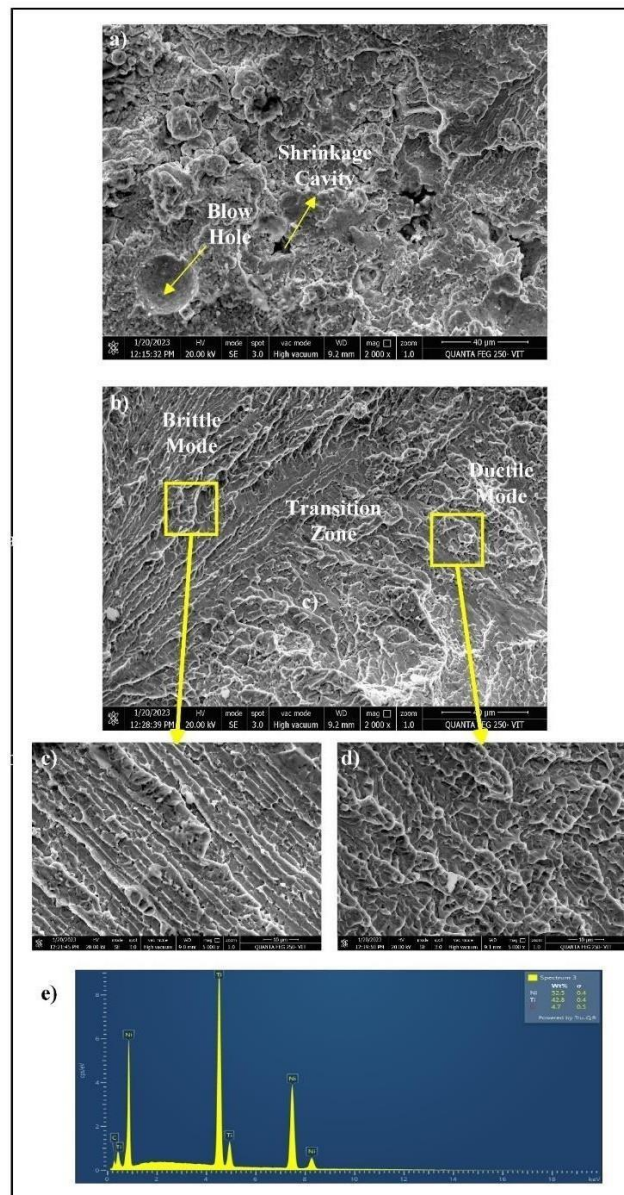
Figure 11. SEM analysis of fractured surface
