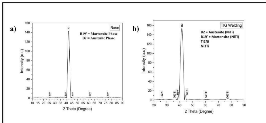
Figure 10: XRD graphs of base metal and TIG Welded sample(75 A, 17cm/min)
